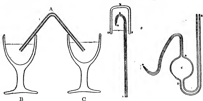
Cavendish's Simple Apparatus in Which the First Nitrogen Fixation Experiment Was Made
